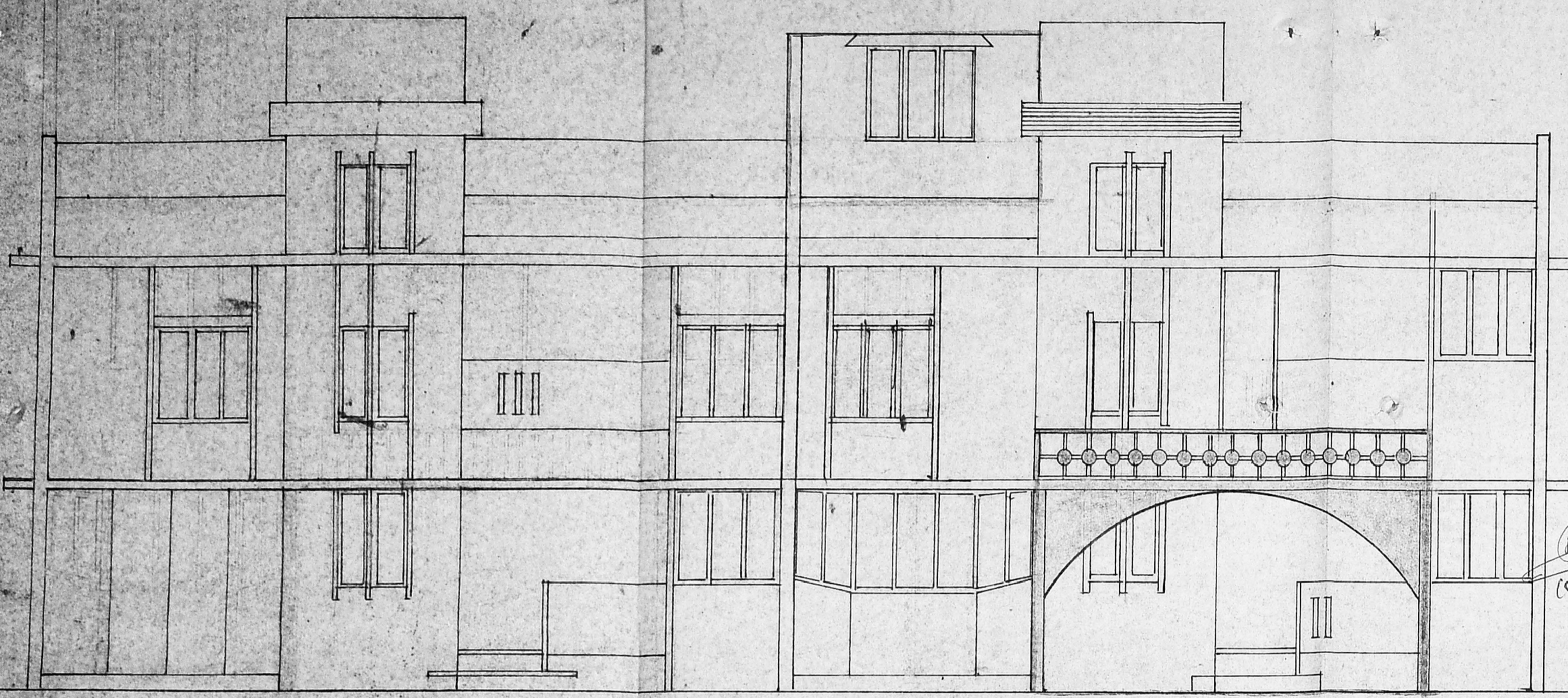
FRONT ELEVATION
